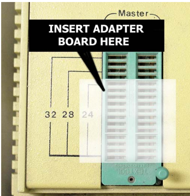
Typical PROM burner socket
