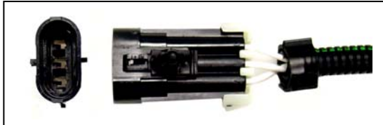
109022 (12") 109023 (24") GM 1994-up 3-wire MAF extension
